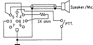
6. Internal connection
