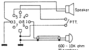
3. External microphone
