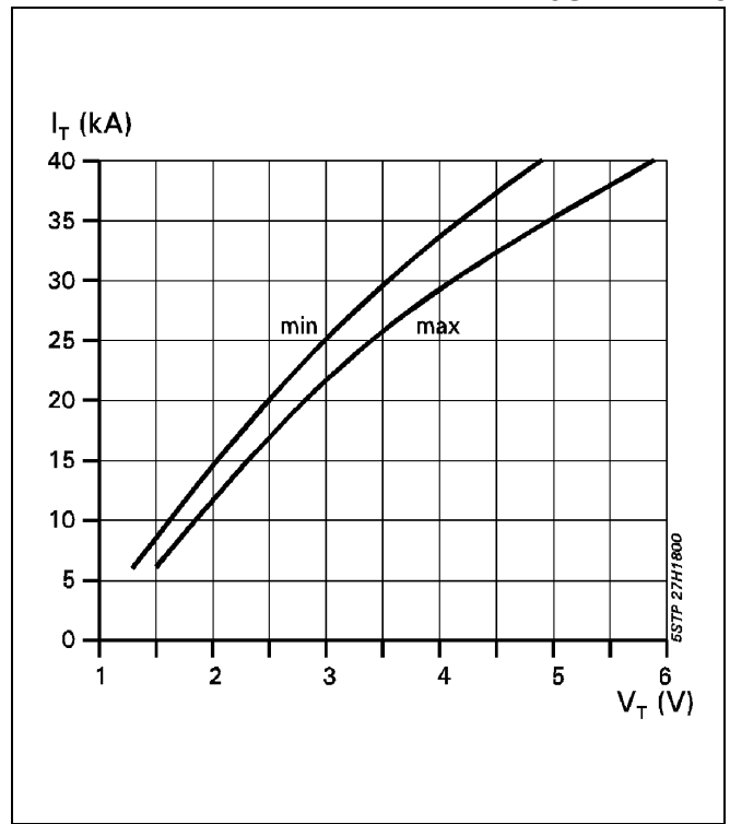
Fig. 3 On-state characteristics. T j =125°C, 10ms half sine
