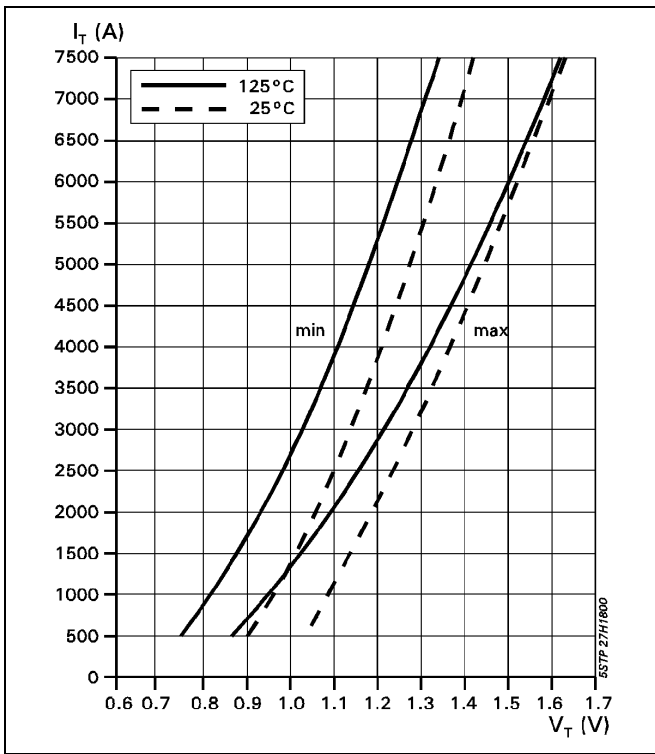
Fig. 2 On-state characteristics.
