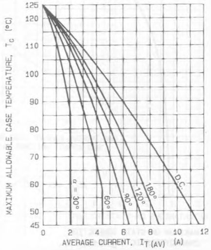
FIG. 2 - MAXIMUM ALLOWABLE CASE TEMPERATURE FOR SIMUSOIDAL CURRENT WAVEFORM
