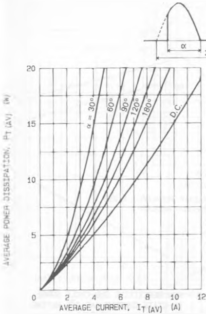
FIG. 1 - MAXIMUM ON-STATE POWER DISSIPATION FOR SIMUSOIDAL CURRENT WAVEFORM
