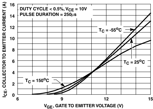
FIGURE 13. TRANSFER CHARACTERISTIC
