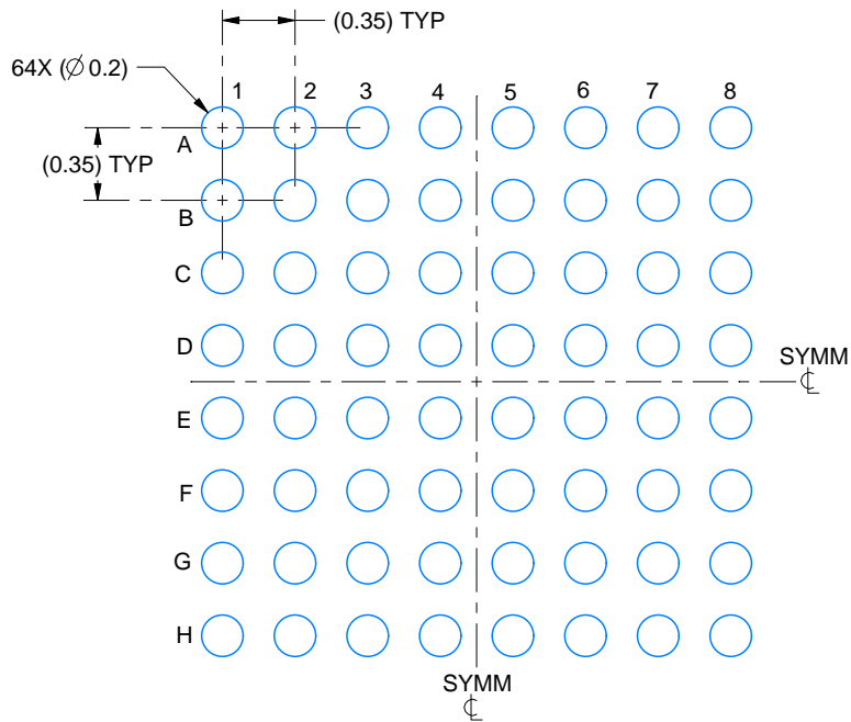
LAND PATTERN EXAMPLE EXPOSED METAL SHOWN SCALE:25X
