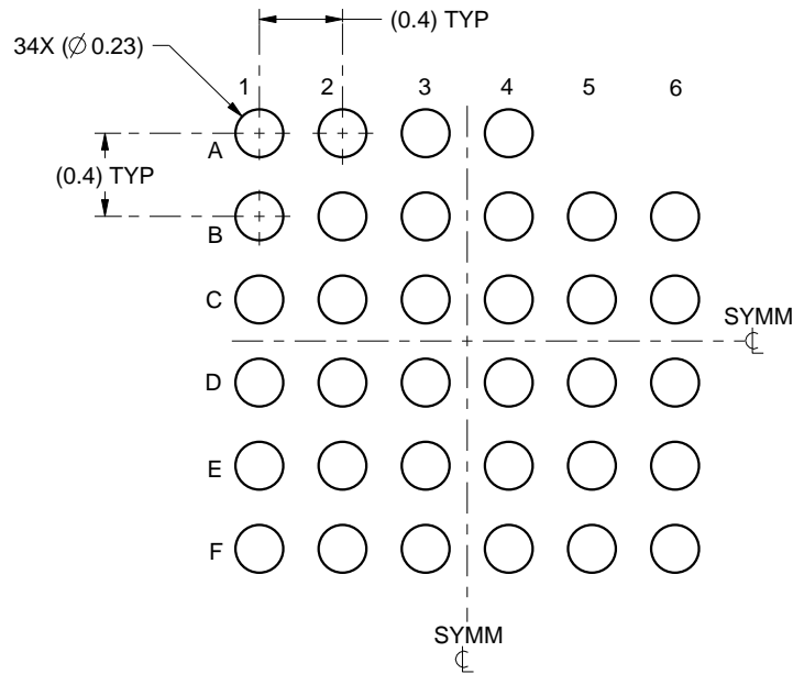
LAND PATTERN EXAMPLE SCALE:25X
