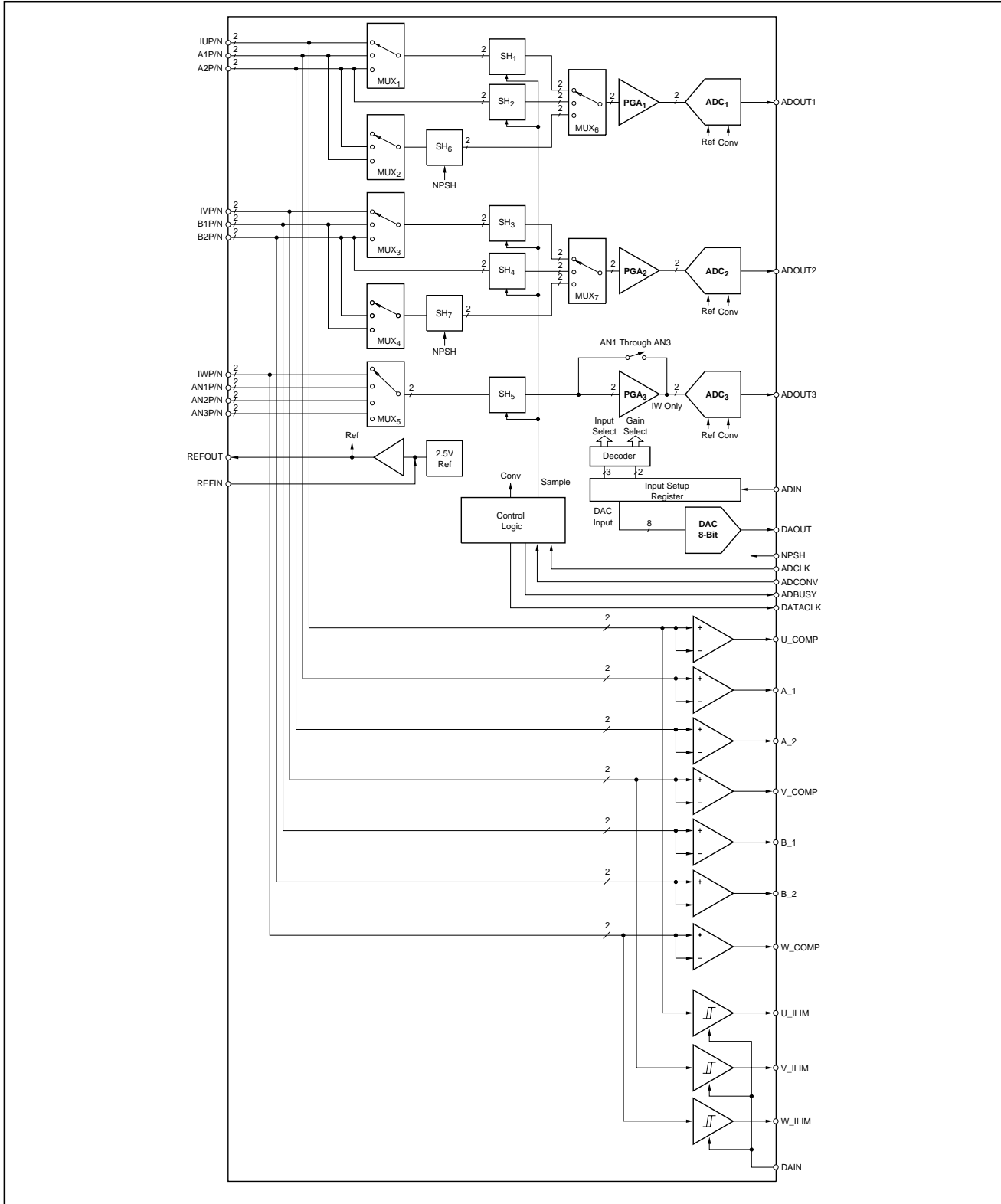
FIGURE 1. Functional Diagram.
