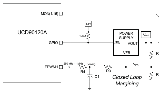
Figure 19. Closed-Loop Margining
