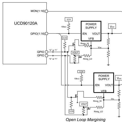
Figure 18. Open-Loop Margining
