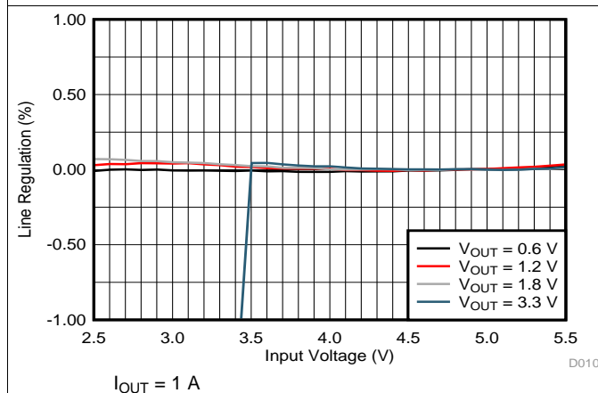
Figure 15. Line Regulation
