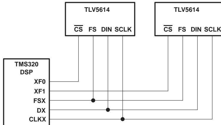
Figure 16. TMS320™ Interface
