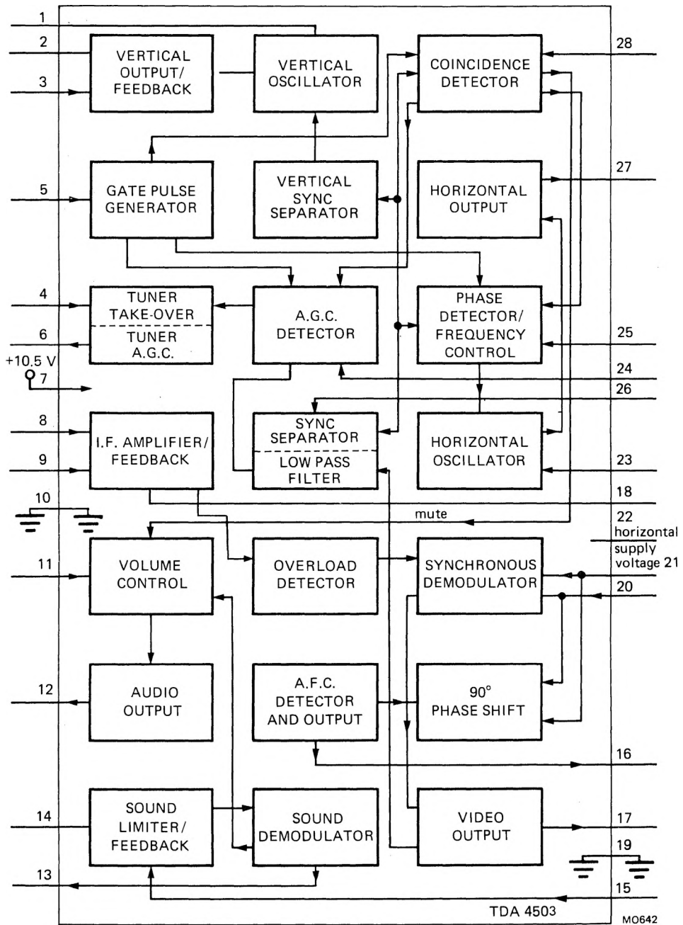
Fig. 1 Block diagram.
