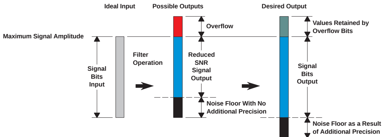
Figure 2-10. TAS5508A Digital Audio Processing
