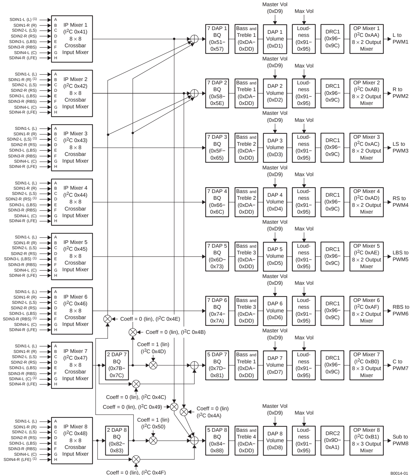
Figure 2-1. TAS5508A DAP Architecture With I²C Registers ( f_s \leq 96 kHz)
