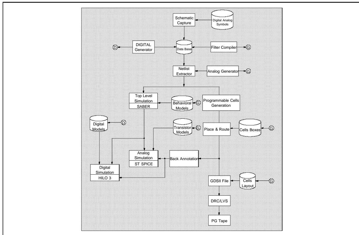
Figure 3: Analog Design System (A.D.S.) flow
