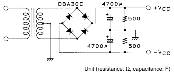
Specified Transformer Power Supply (RP-25 equivalent)
