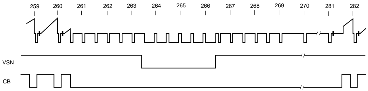
(b) 2nd field CVBS output signal
