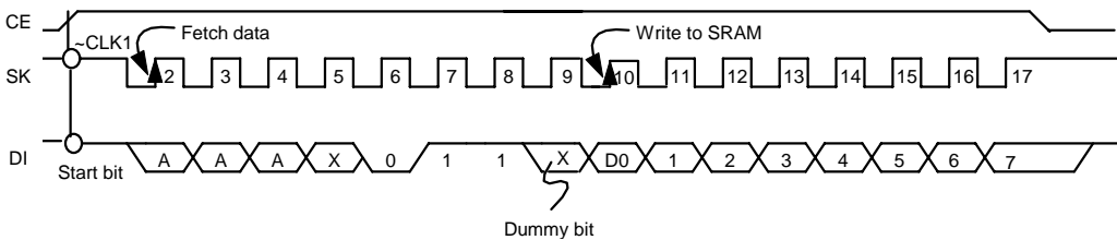
Figure 16 Write mode timina(S-24H30, S-24S30)
