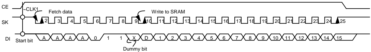
Figure 15 Write mode timing(S-24H45, S-24S45)
