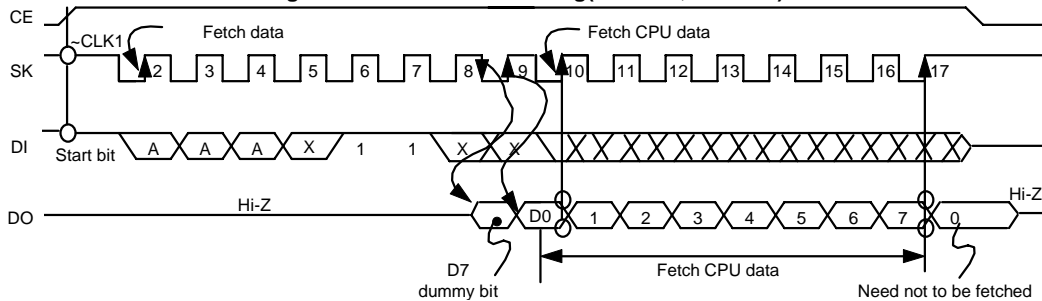
Figure 13 Read mode timing(S-24H45, S-24S45)
