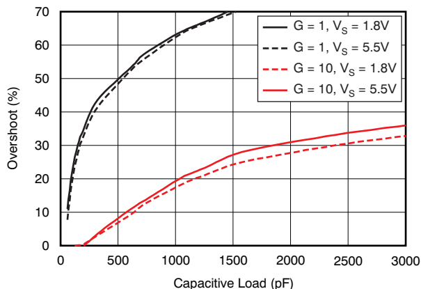
Figure 33. Small-Signal Overshoot versus Capacitive Load ( 100\text{mV}_{\text{pp}} output step)
