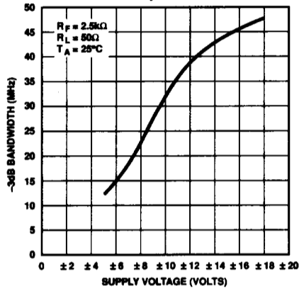
SMALL-SIGNAL -3dB BANDWIDTH vs SUPPLY VOLTAGE A_V = +1
