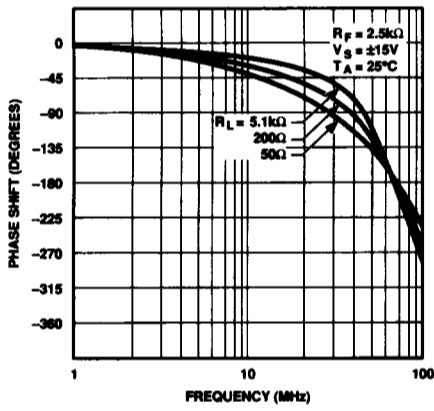
PHASE SHIFT vs FREQUENCY A_V = +2
