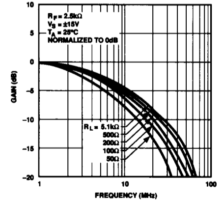
GAIN vs FREQUENCY A_V = +50
