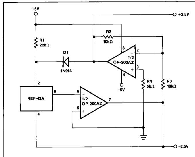
FIGURE 5. Dual Precision Voltage Reference
