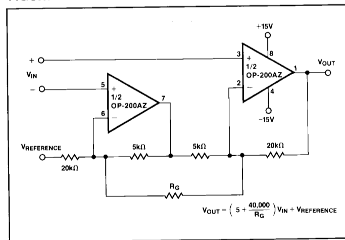
FIGURE 1: Dual Low-Power Instrumentation Amplifier
