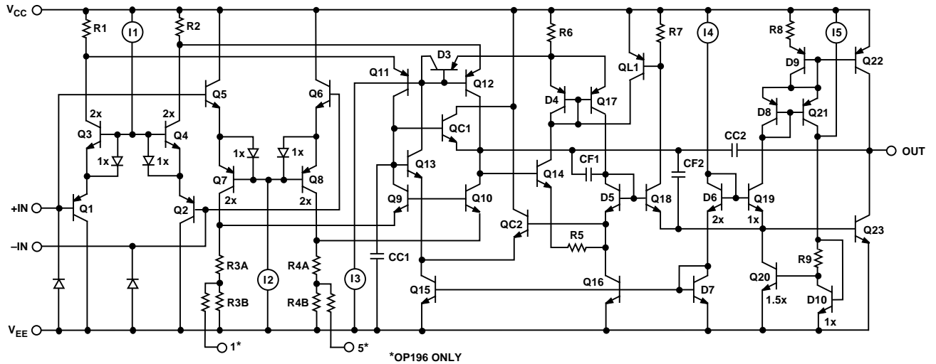
Figure 36. Simplified Schematic
