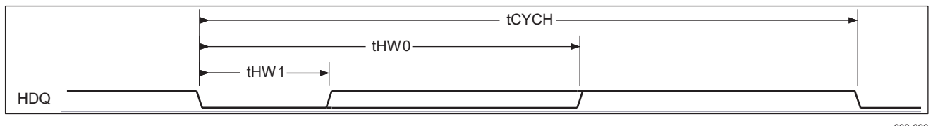
Figure 6-56. HDQ Read Bit Timing (Data)
