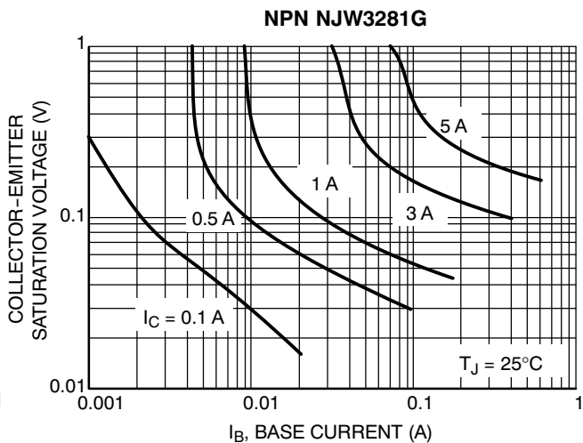
Figure 8. Saturation Region
