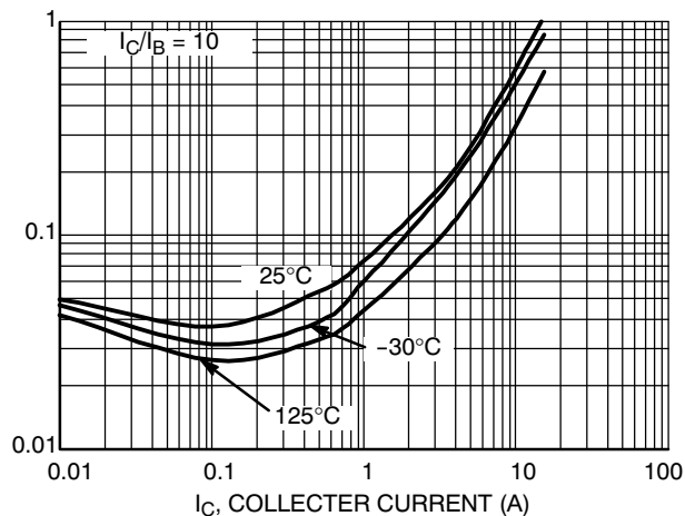
Figure 10. V_{CE(sat)} , Collector-Emitter Saturation Voltage
