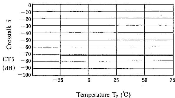
Crosstalk 5 vs. Temperature ( V^+ = 5\text{ V} )
