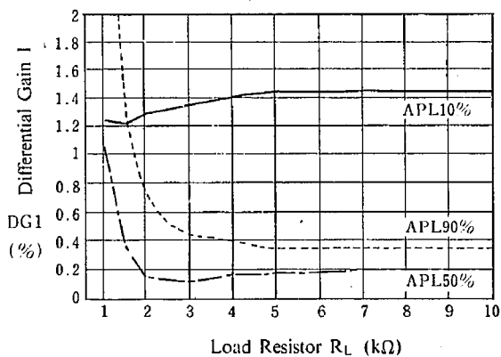
Differential Gain 1 vs. Load Resistor
