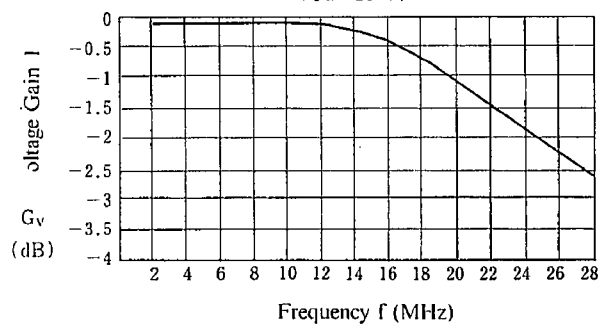
Voltage Gain 1 vs. Frequency
