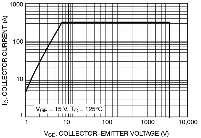
Figure 18. Reverse Bias Safe Operating Area
