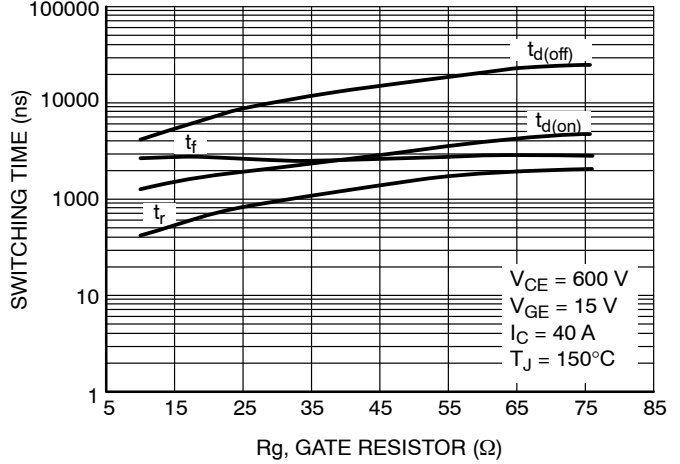
Figure 14. Switching Time vs. Rg
