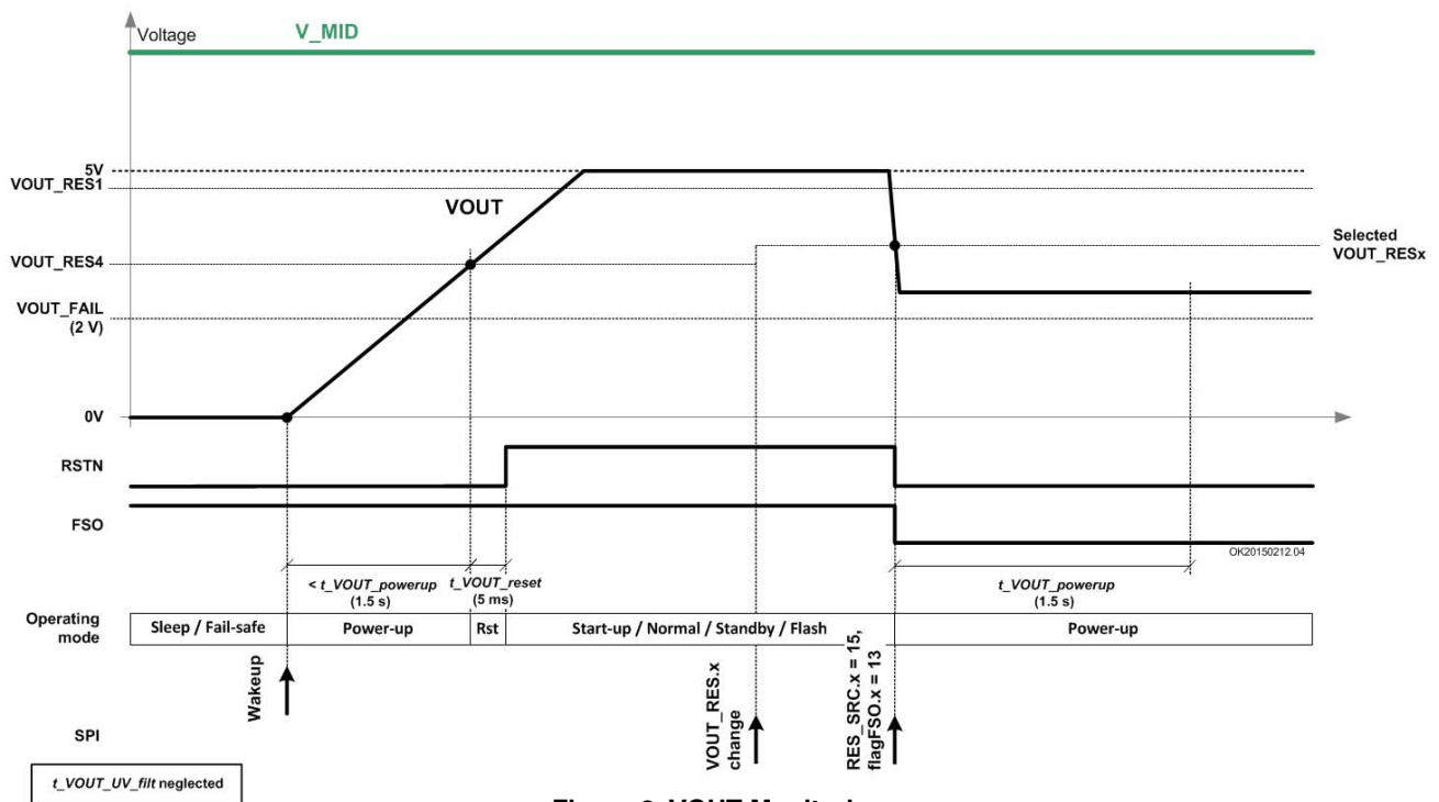
Figure 6. VOUT Monitoring
