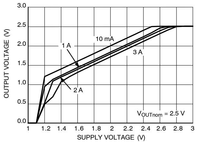
Figure 7. Dropout Characteristics
