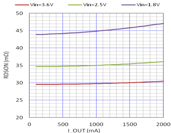
Figure 9. R_{DS(on)} (mΩ) vs. Current (mA)
