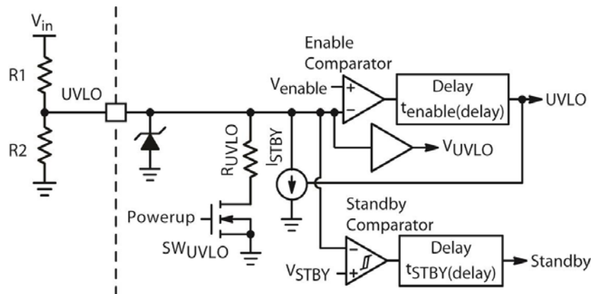
Figure 9. UVLO Block Diagram
