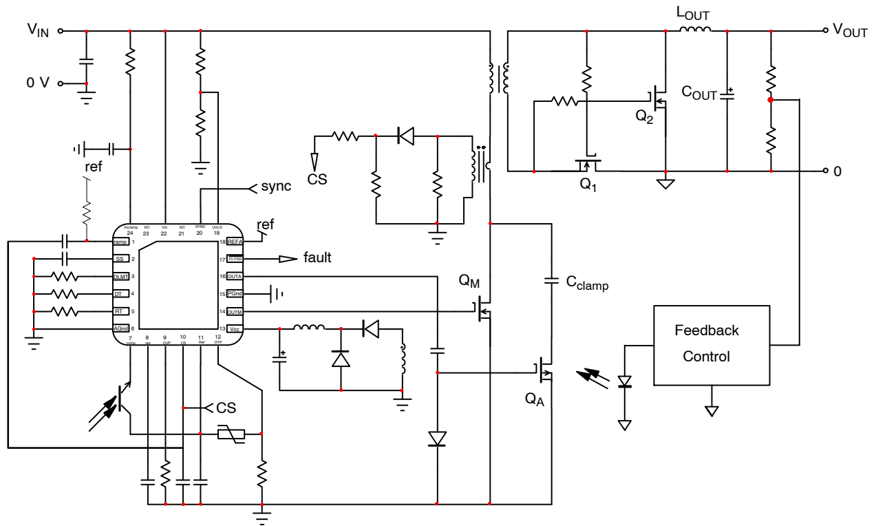
Figure 2. Typical Application Circuit in Current Mode Control
