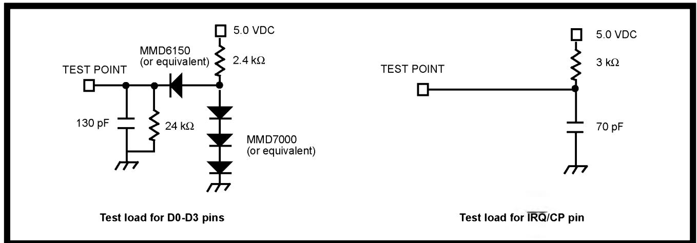
Figure 14 - Test Circuit
