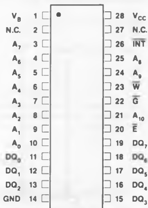
FIGURE 1. PIN CONNECTIONS
