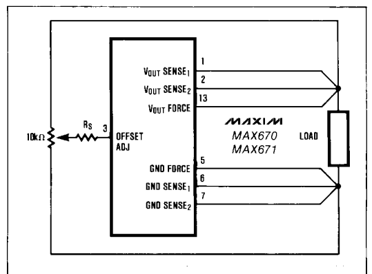
Figure 9. MAX670/671 Improved TC Independent Trim Adjustment
