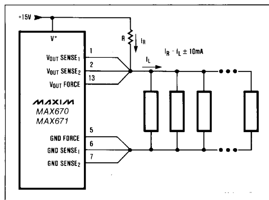
Figure 8. Pull Up Resistor Load Balancing
