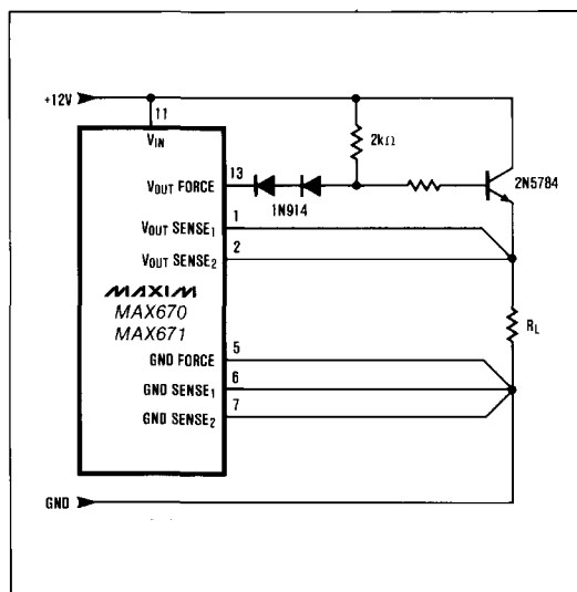
Figure 5. Application Circuit for 12V Operation, 120mA Output Current
