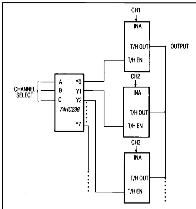
Figure 3. MAX271 Multiplexed Operation
