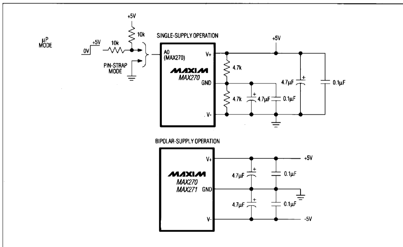
Figure 4. Power-Supply Configurations
