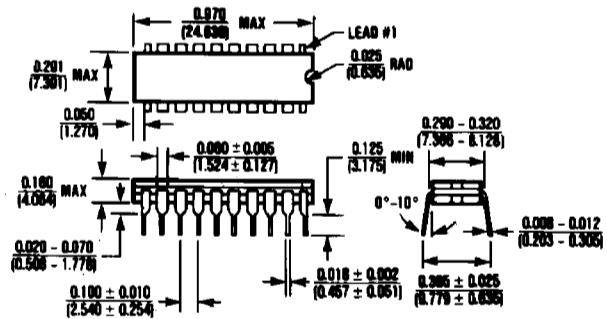
20 Lead Cerdip
