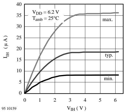
Figure 35. All PINs with pull-down: n-channel sink current
