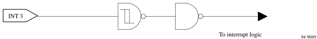
Figure 12. External interrupt input
