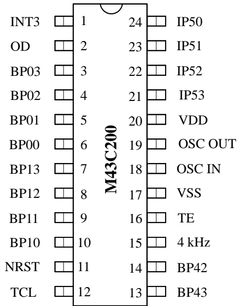
Figure 2. Pin assignment SO24 (top view)
