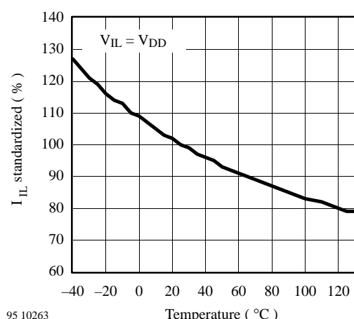
Figure 39. Standardized n-channel sink current vs. ambient temperature
