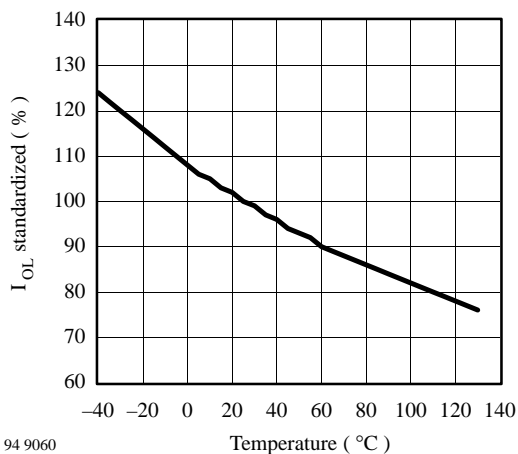
Figure 23. Standardized n-channel sink current vs. ambient temperature
