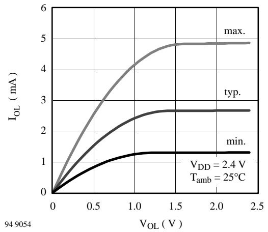
Figure 17. N-channel sink current
