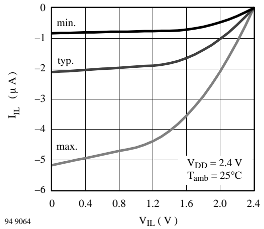
Figure 27. PIN NRST: p-channel source current
