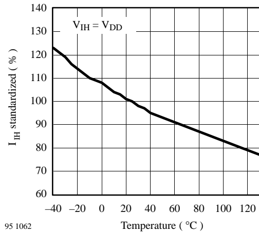
Figure 38. Standardized p-channel source current vs. ambient temperature
