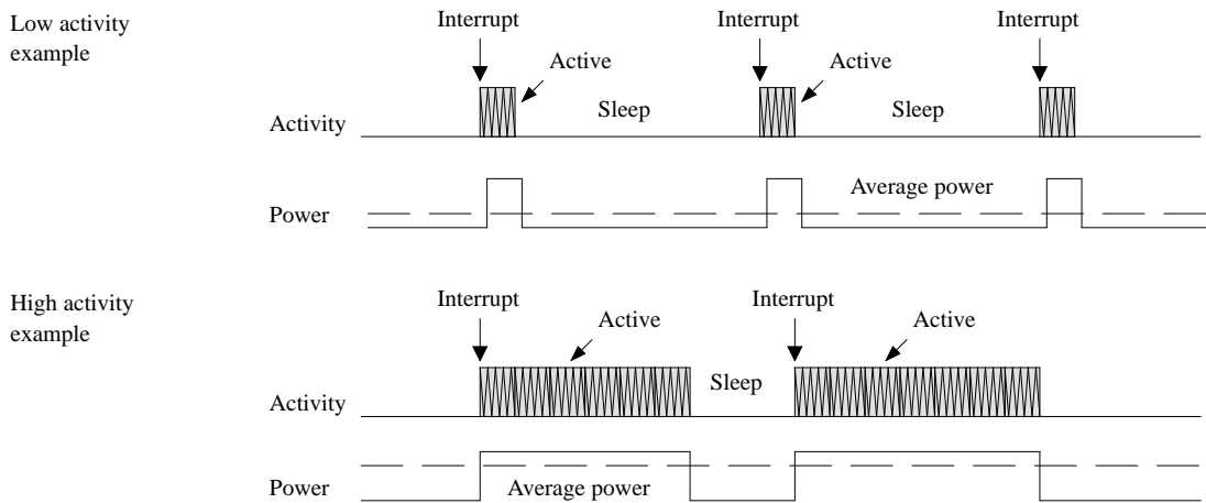
Figure 13. Average system power consumption and duty cycle
