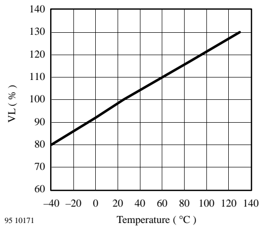
Figure 47. Typical switch level vs. ambient temperature
