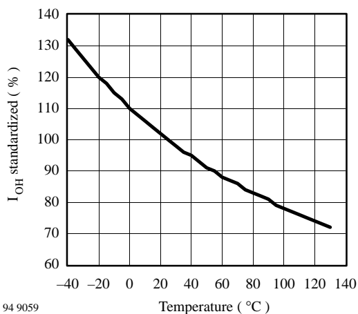
Figure 22. Standardized p-channel source current vs. ambient temperature
