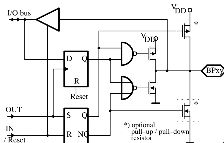
Figure 4. Bidirectional port schematics
