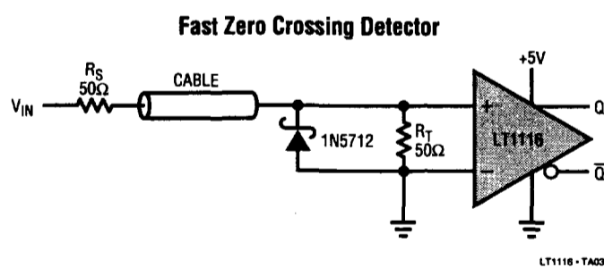
Figure 1. The zero crossing detector terminates the transmission line at its 50Ω characteristic impedance. Negative inputs should not fall below -2V to keep the signal current within the clamp diode's maximum forward rating. Positive inputs should not exceed the device's absolute maximum ratings nor the power rating on the terminating resistor.
