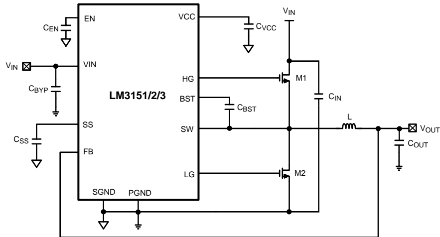
Figure 5. Design Example Schematic
