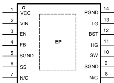
Figure 1. eTSSOP-14
