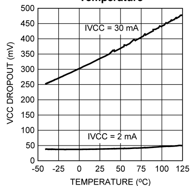
VCC Dropout vs. Temperature
