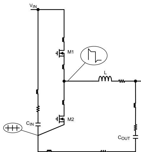
Figure 6. Schematic of Parasitics
