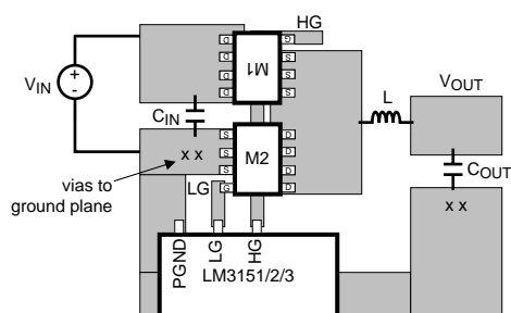
Figure 7. PCB Placement of Power Stage
