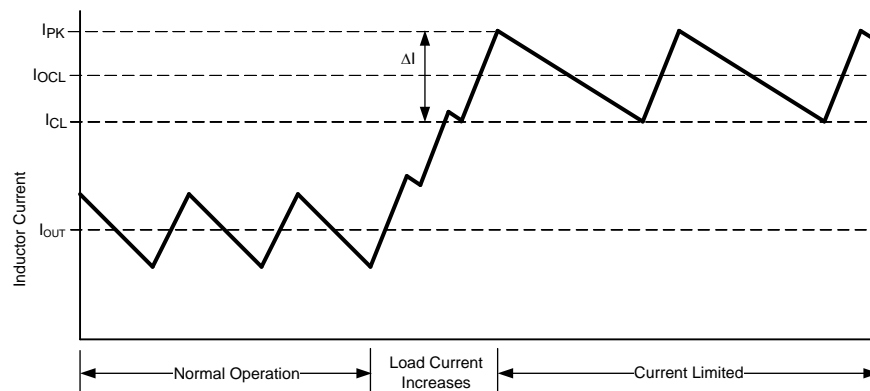
Figure 2. Inductor Current - Current Limit Operation
