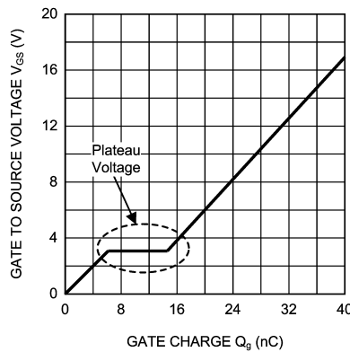
Figure 4. Typical MOSFET Gate Charge Curve
