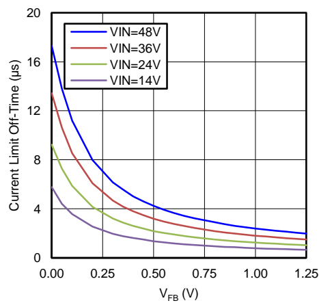
Figure 8. T OFF (I LIM ) vs V FB and V IN
