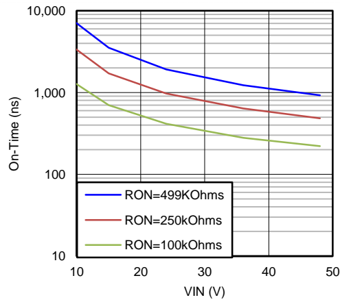
Figure 7. T ON vs V IN and R ON
