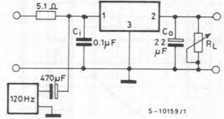
Fig. 3 - Ripple Rejection
