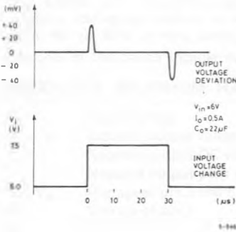
Fig. 16 - Line transient response
