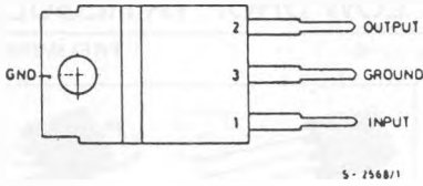
TO-220
