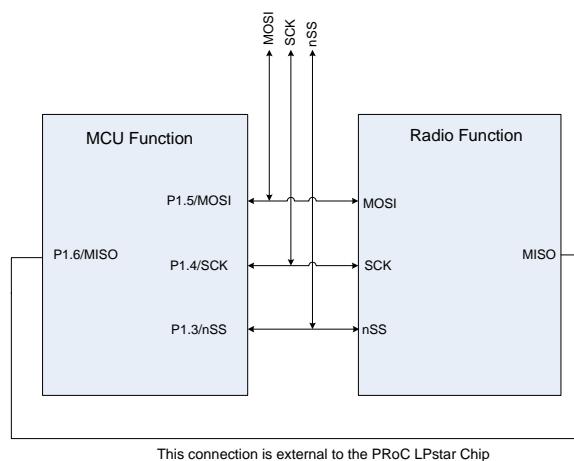
Figure 5. Four-Wire SPI Mode
