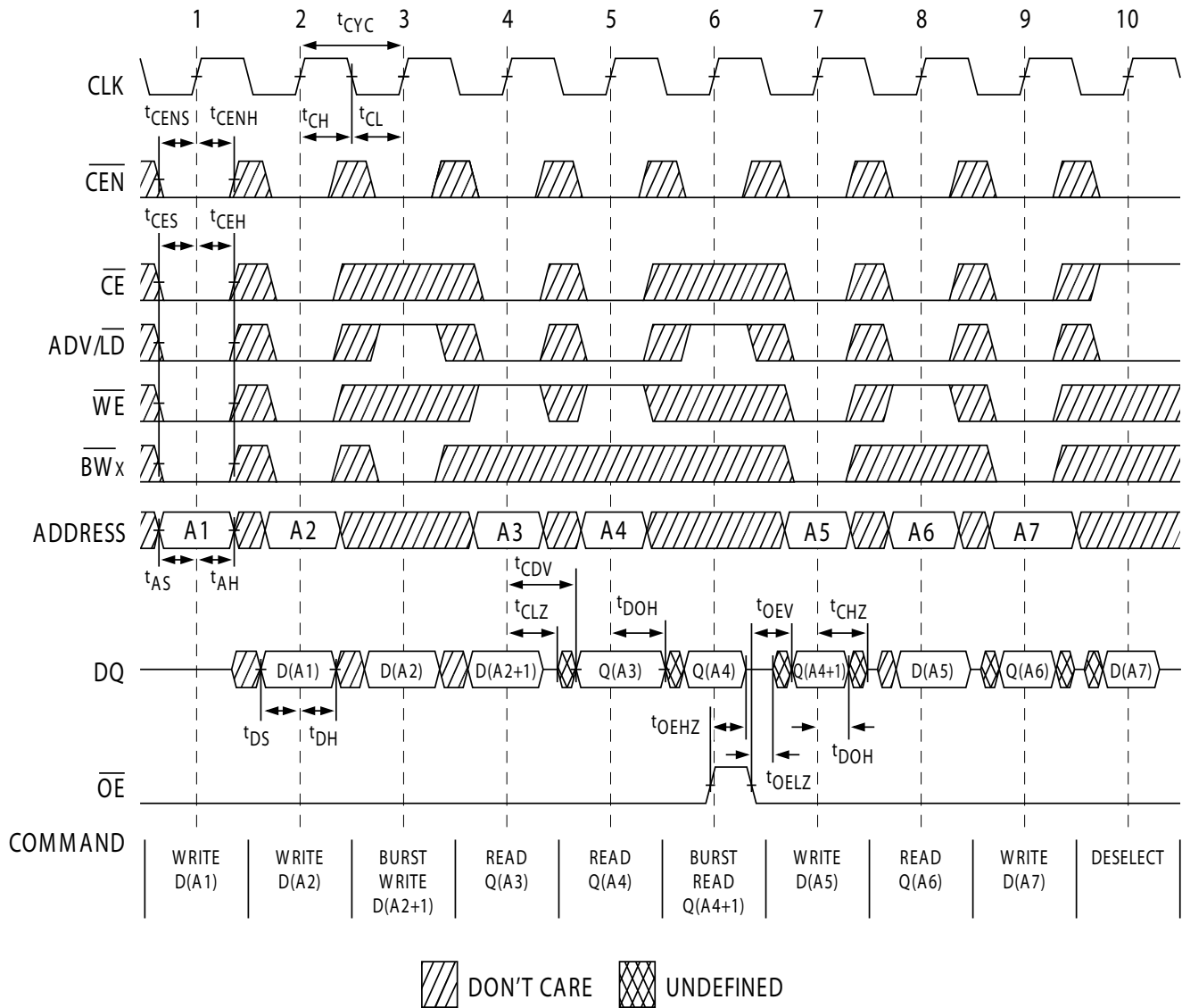
Figure 7. Read/Write Waveforms [28, 29, 30]
