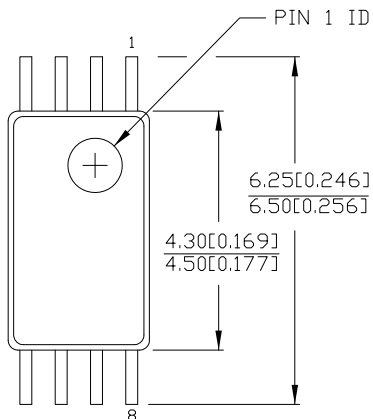
Figure 13. 8-Pin Thin Shrunk Small Outline Package (4.40 MM Body) Z8
