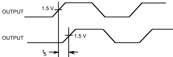
Figure 4. Output-Output Skew
