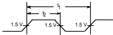
Figure 3. All Outputs Rise/Fall Time
