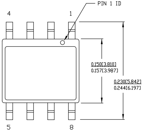
Figure 10. 8-Pin (150-Mil) SOIC S8
