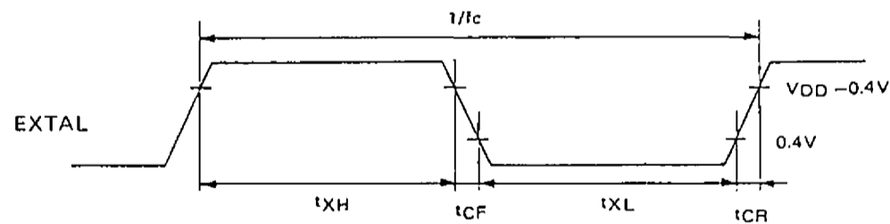
Fig. 1. Clock timing
