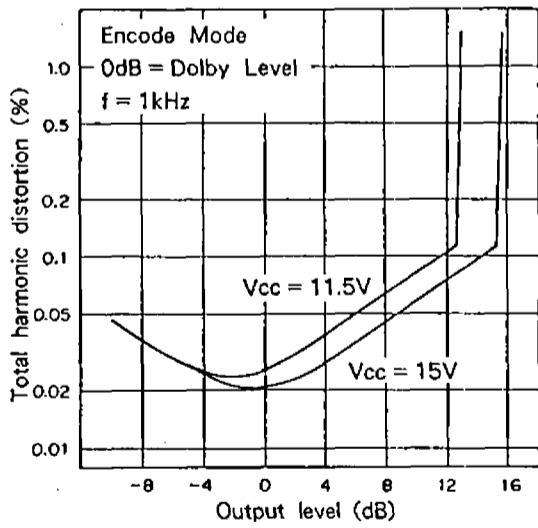
B type total harmonic distortion-2 (CXA1330)
