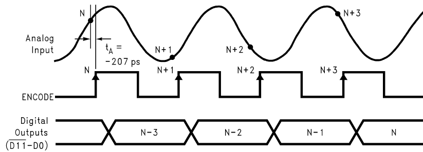
CLC5956 Aperture Delay Diagram
