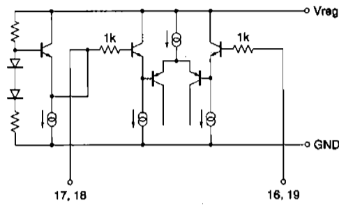
(4) I/O of amplifiers 1 and 2
