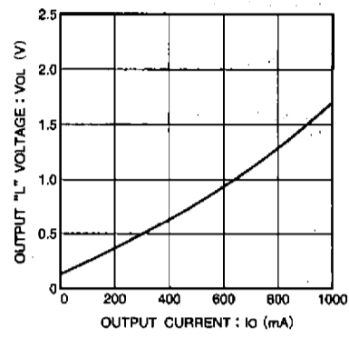
Fig.15 LOW level output voltage vs. output current
