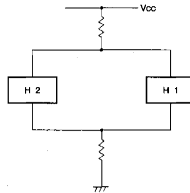
Parallel connection
