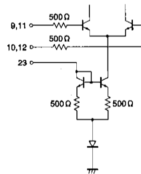
(3) Hall input (9, 10, 11, 12 pin) and E_{ci} input
