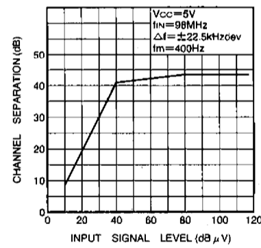
Fig. 26 Sensitivity characteristics
