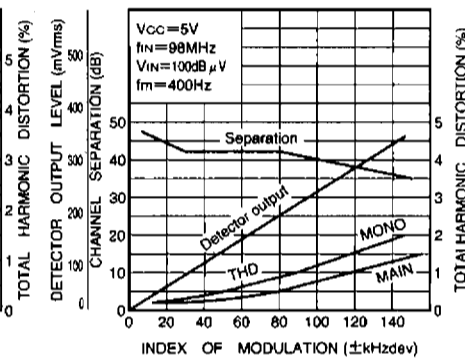
Fig. 23 Modulation characteristics
