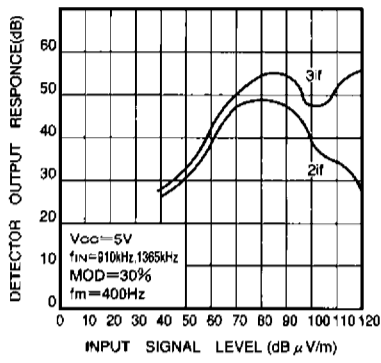
Fig. 18 Beat characteristics
