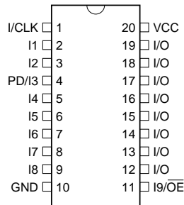
DIP/SOIC
