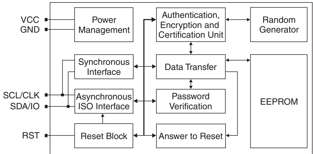
Figure 1. Block Diagram
