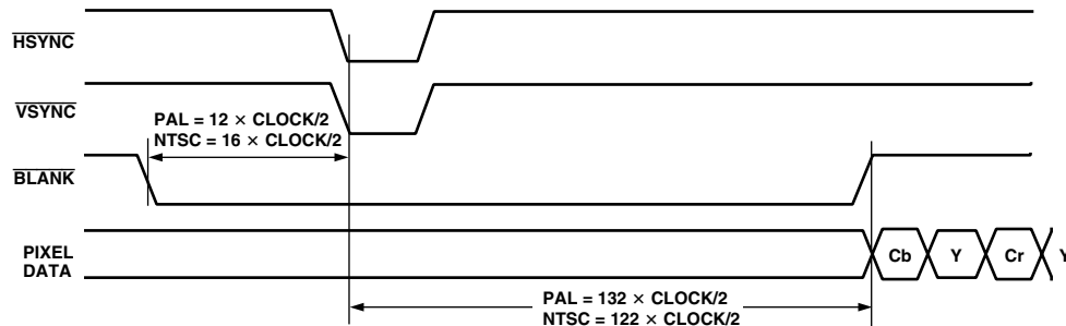
Figure 42. Timing Mode 2, Even-to-Odd Field Transition Master/Slave
